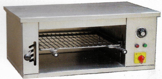
RPF 4 Salamander - Electric Major O/S 910 X 535 X 360 mm Minor O/S 740 X 500 X 322 mm
