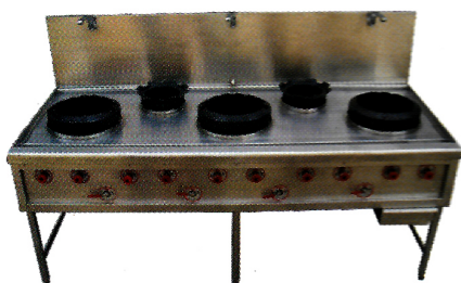
RC 16 Chinese Cooking Range O/S 900 X 900 X 850 + 450 mm (1 Main Burner & 1 Stock Burner) O/S 1500 X 900 X 850 + 450 mm (2 Main Burner & 1 Stock Burner) O/S 2100 X 900 X 850 + 450 mm (3 Main Burner & 2 Stock Burner)
