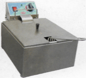
RPF 3A Mini Master Fryer (Single Tank) Capacities: 5 Ltrs- O/S 188 x 421 x (210 + 100) mm 8 Ltrs- O/S 280 x 421 x (210 + 100) mm
