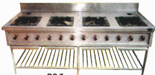
RC 7 Four Burner Range with Slimmer Plate O/S 2100 X 900 X 850 + 150 mm
