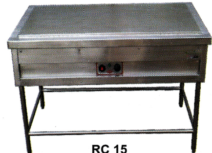
RC 15 Electric Range O/S 1500 X 600 X 850 mm
