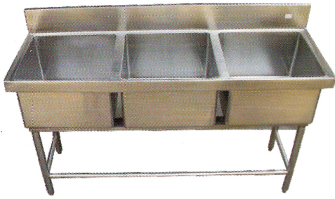
RW 1 3 Sink Dish Wash Unit O/S 1800 X 600 X 850 + 150 mm O/S 2100 X 600 X 850 + 150 mm
