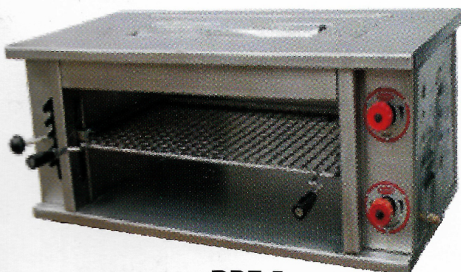
RPF 5 Salamander - Gas O/S 910 X 535 X 350 mm
