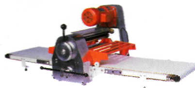
RB 5 Dough Sheeter Table Top model O/S 1800 X 900 X 600 mm Floor model O/S 2100 X 900 X 1100 mm
