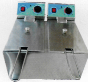
RPF 3B Mini Master Fryer (Double Tank) Capacities: 5 + 5 Ltrs- O/S 385 x 421 x (210 + 100) mm 8 + 8 Ltrs- O/S 567 x 421 x (210 + 100) mm
